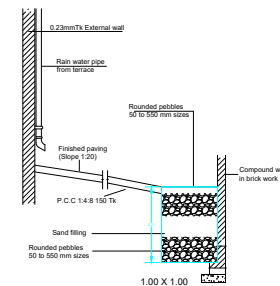
PLAN OF RAIN WATER HARVESTING
