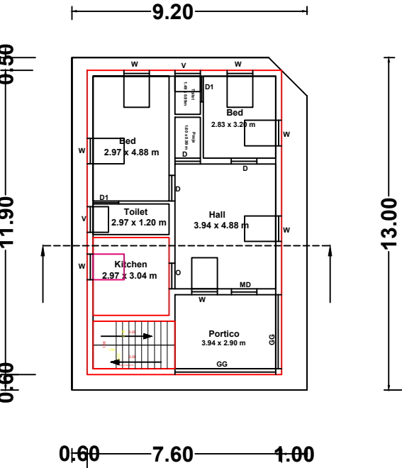
GROUND FLOOR PLAN ( EXISTING )
