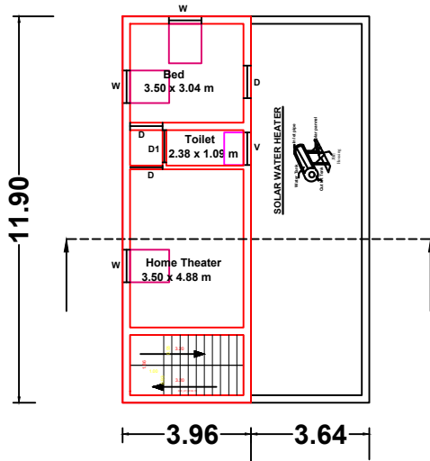
SECOND FLOOR PLAN ( PROPOSED ) & TERRACE FLOOR PLAN
