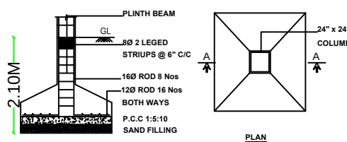
FOUNDATION DETAILS
