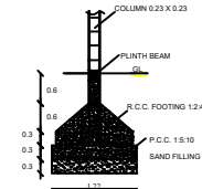
COLUMN DETAILS
