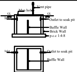
PLAN SEPTIC TANK
