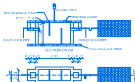
SEPTIC TANK AND TRENCH & U TRAP ADOPTED
