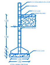
COLUMN SECTION
