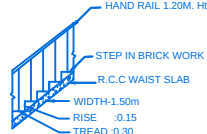
STAIR DETAIL
