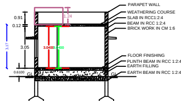
SECTIONAL ELEVATION ON A-A
