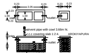
Details of septic tank & trench
