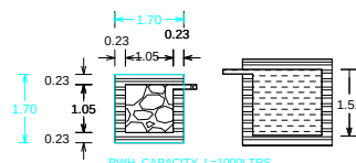
DETAILS OF FILTER BED & WELL
