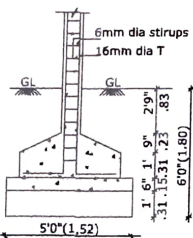
COLUMN FOUNDATION DETAIL
