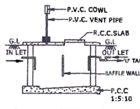
SEC. OF SEPTIC TANK
