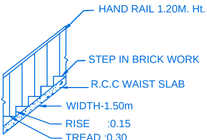
STAIR DETAIL
