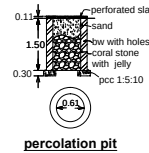
percolation pit
