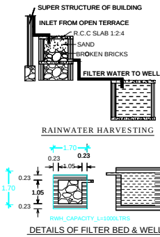
DETAILS OF FILTER BED & WELL
