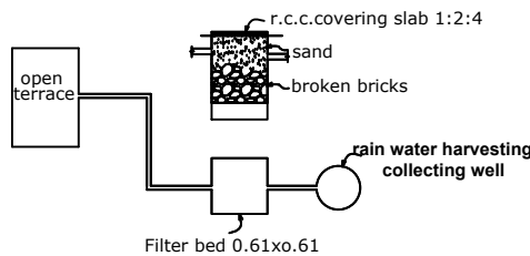
Details of rain water harvesting system
