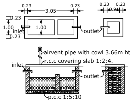
Details of septic tank & trench
