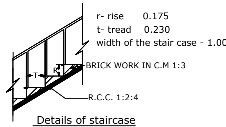
Details of staircase
