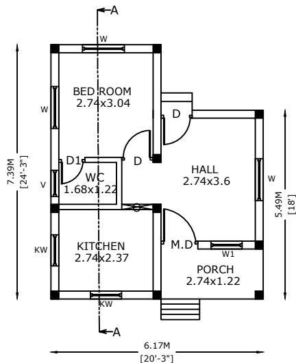
PRO.GROUND FLOOR
