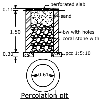
Percolation pit
