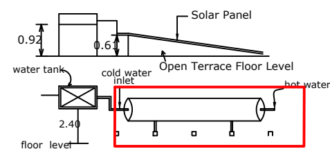
Details of solar water harvesting system
