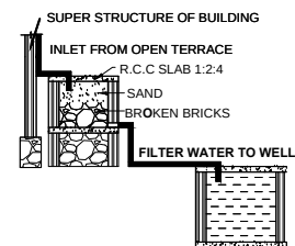
RAINWATER HARVESTING
