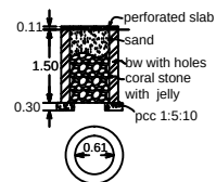
percolation pit
