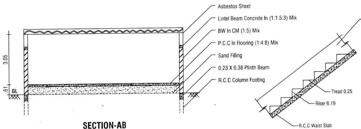
STAIR DETAILS
