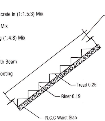
STAIR DETAILS
