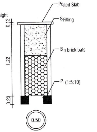
RAIN WATER COLLECTION WELL
