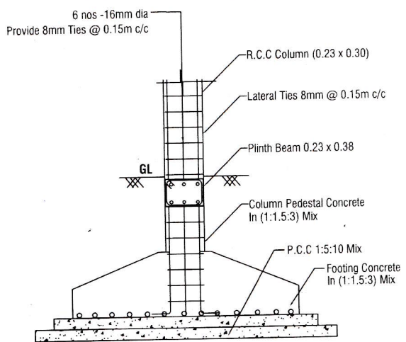
COLUMN FOOTING DETAILS
