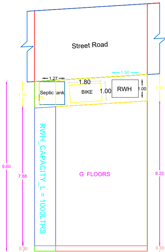
SITE PLAN
