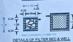
RAINWATER HARVESTING
