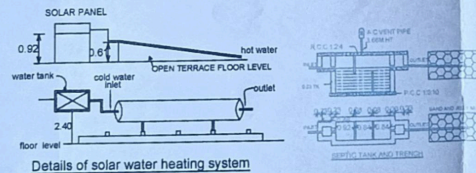
Details of solar water heating system
