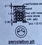
percolation pit
