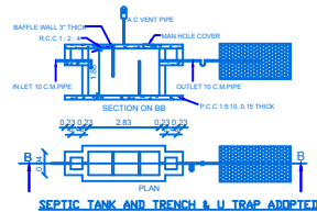
SEPTIC TANK AND TRENCH & U TRAP ADOPTED
