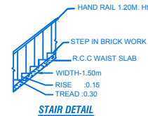
STAIR DETAIL
