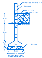
COLUMN DETAIL
