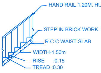
STAIR DETAIL
