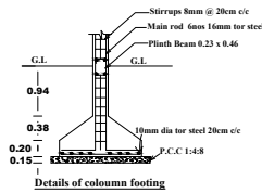
Details of column footing
