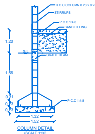
COLUMN DETAIL
