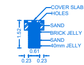
SECTION OF RAIN WATER COLLECTION TANK
