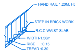
STAIR DETAIL
