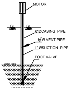
SEC. OF BOREWELL
