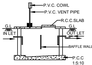
SEC. OF SEPTIC TANK
