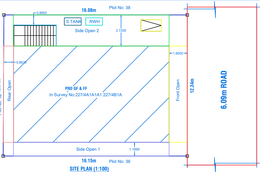
SITE PLAN (1:100)
