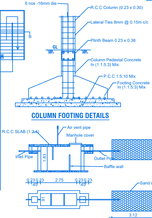
SEPTIC TANK & TRENCH
