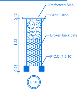
RAIN WATER COLLECTION WELL
