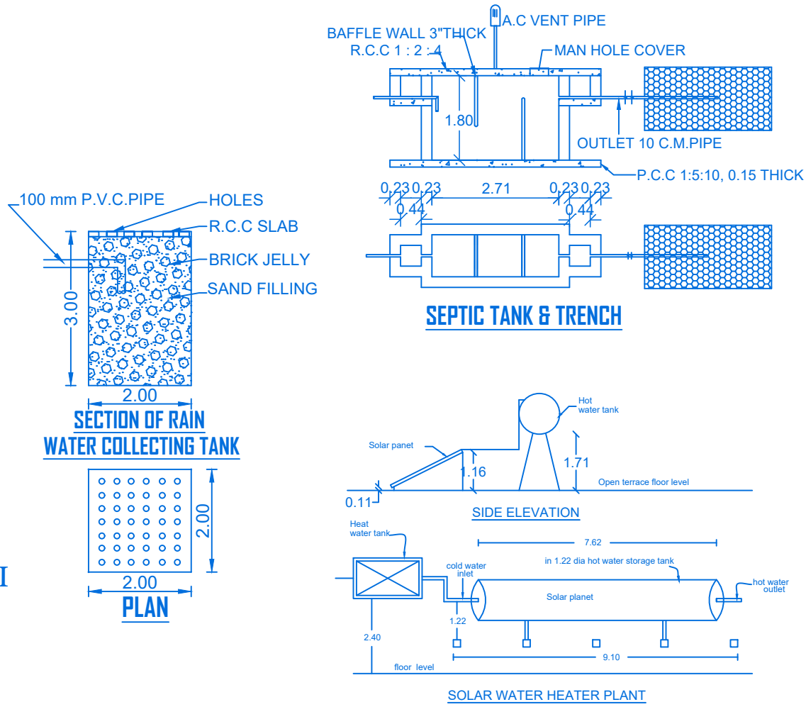
SOLAR WATER HEATER PLANT
