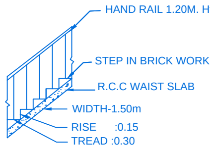
STAIR DETAIL
