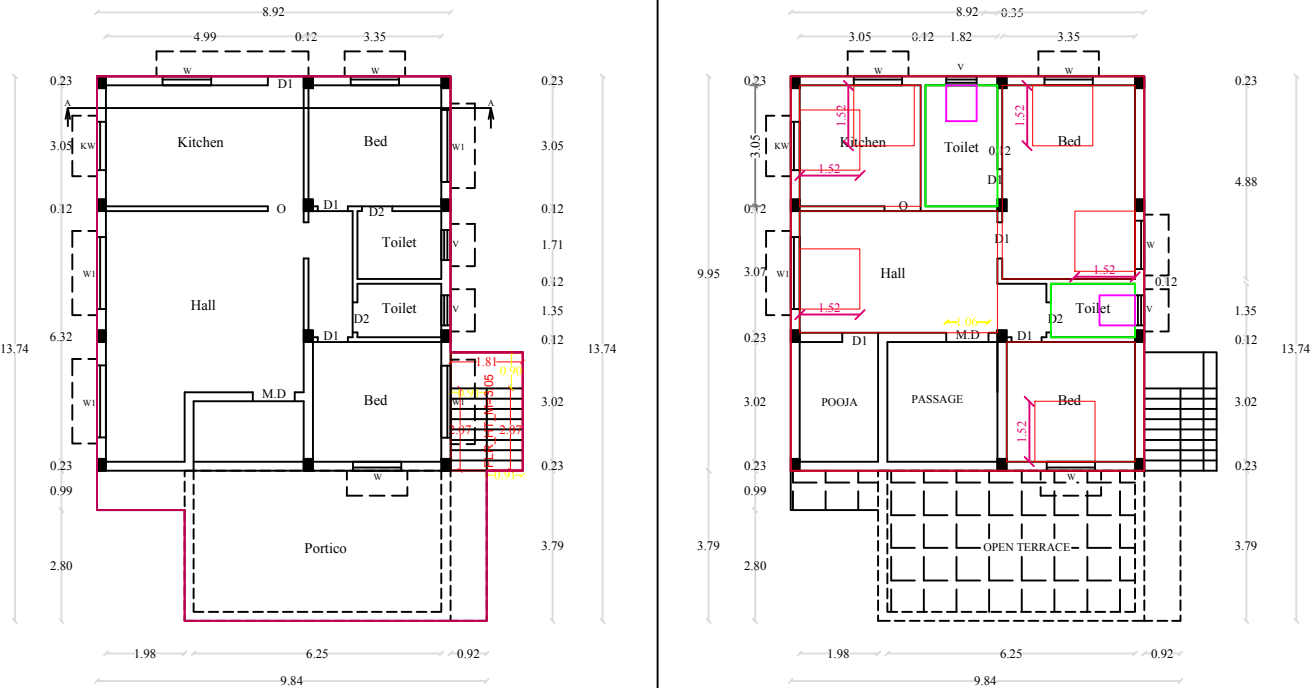
EXG.GROUND FLOOR PLAN
