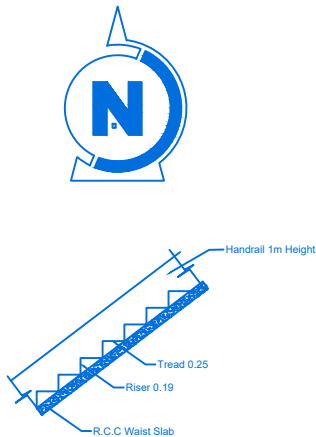
STAIR DETAILS
