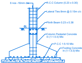
COLUMN FOOTING DETAILS
