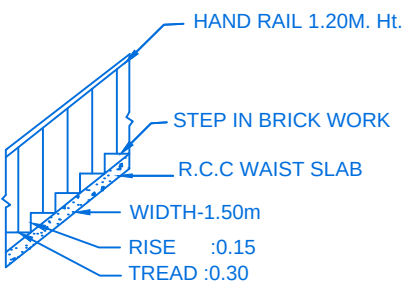
STAIR DETAIL
