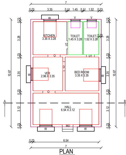
PLAN
