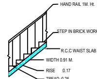
STAIR DETAIL
