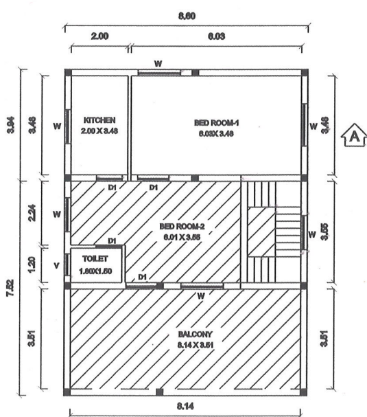
PROPOSED ADDITIONAL FIRST FLOOR PLAN
