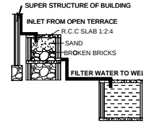
RAINWATER HARVESTING
