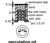
percolation pit
