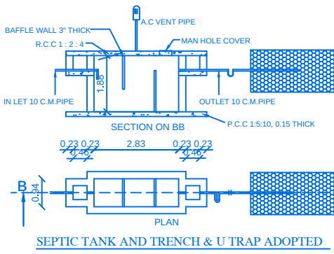
SECTION ON BB
