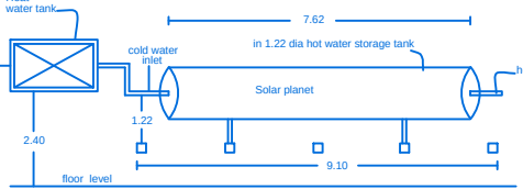
SOLAR WATER HEATER PLANT
