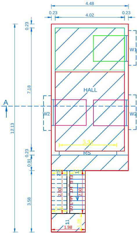
EXG.GROUND FLOOR PLAN
