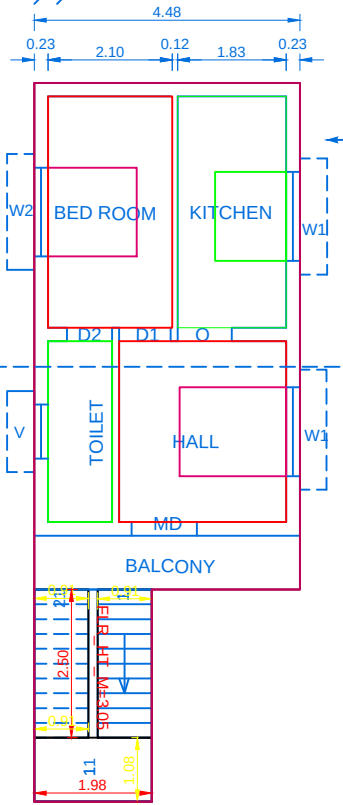
PROP.FIRST FLOOR PLAN
