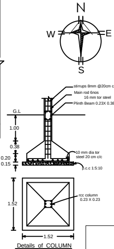
Details of COLUMN
