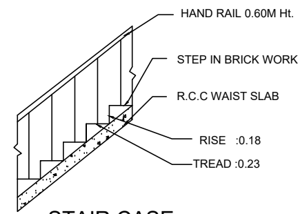
STAIR CASE
