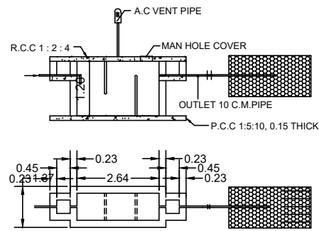
SEPTIC TANK
