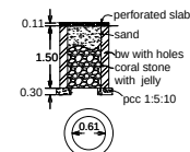
percolation pit
