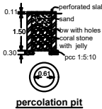
percolation pit
