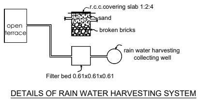
DETAILS OF RAIN WATER HARVESTING SYSTEM
