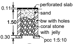
percolation pit
