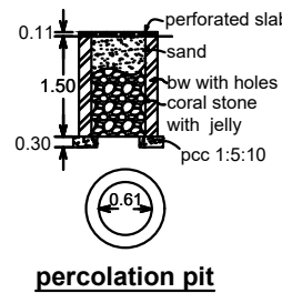
percolation pit
