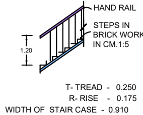
DETAILS OF STAIRCASE
