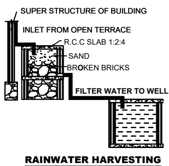
RAINWATER HARVESTING
