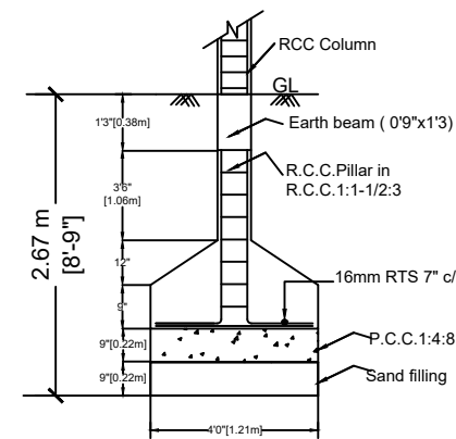
FOUNDATION DETAILS
