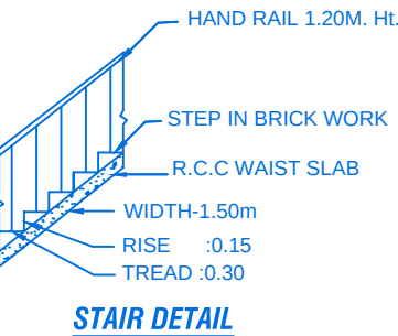
STAIR DETAIL
