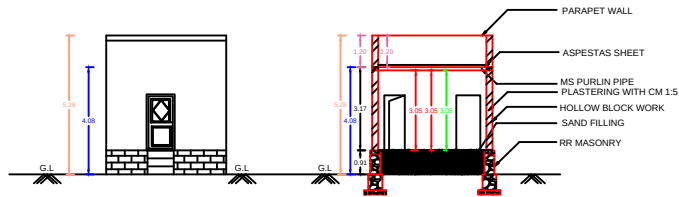
FRONT ELEVATION
