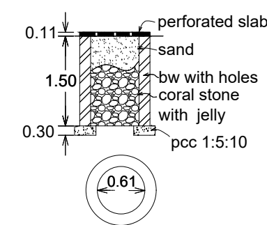
percolation pit
