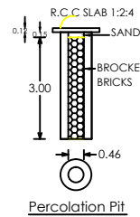
Percolation Pit
