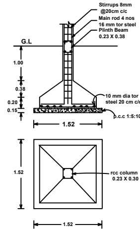
Details of column footing
