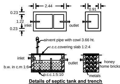
Details of septic tank and trench
