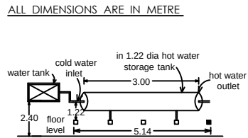
Details of solar hot water system
