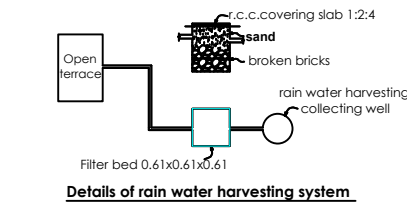
Details of rain water harvesting system
