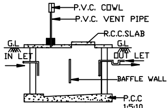
SEC. OF SEPTIC TANK
