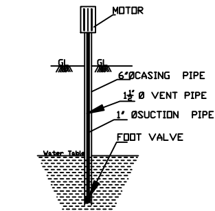
SEC. OF BOREWELL
