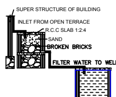
RAINWATER HARVESTING
