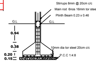
Details of column footing
