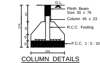
COLUMN DETAILS
