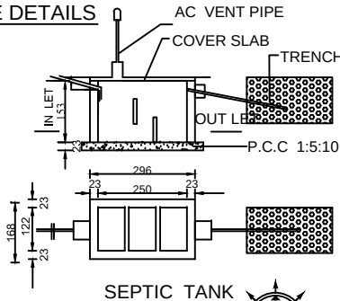
SEPTIC TANK
