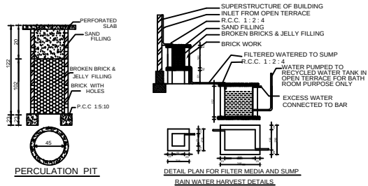
PERCOLATION PIT
