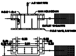
SEPTIC TANK
