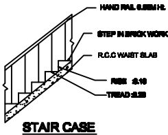
STAIR CASE
