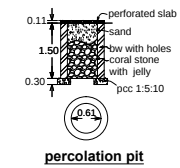
percolation pit
