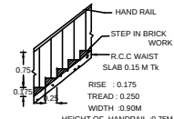
STAIR DETAILS
