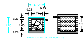
DETAILS OF FILTER BED & WELL
