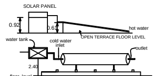
Details of solar water heating system
