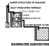
RAINWATER HARVESTING
