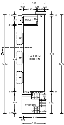
EXG.GROUND FLOOR PLAN
