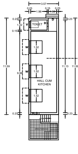
PROP.FIRST FLOOR PLAN
