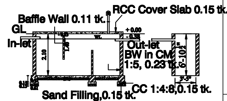
SECTION - SEPTIC TANK NOT TO SCALE
