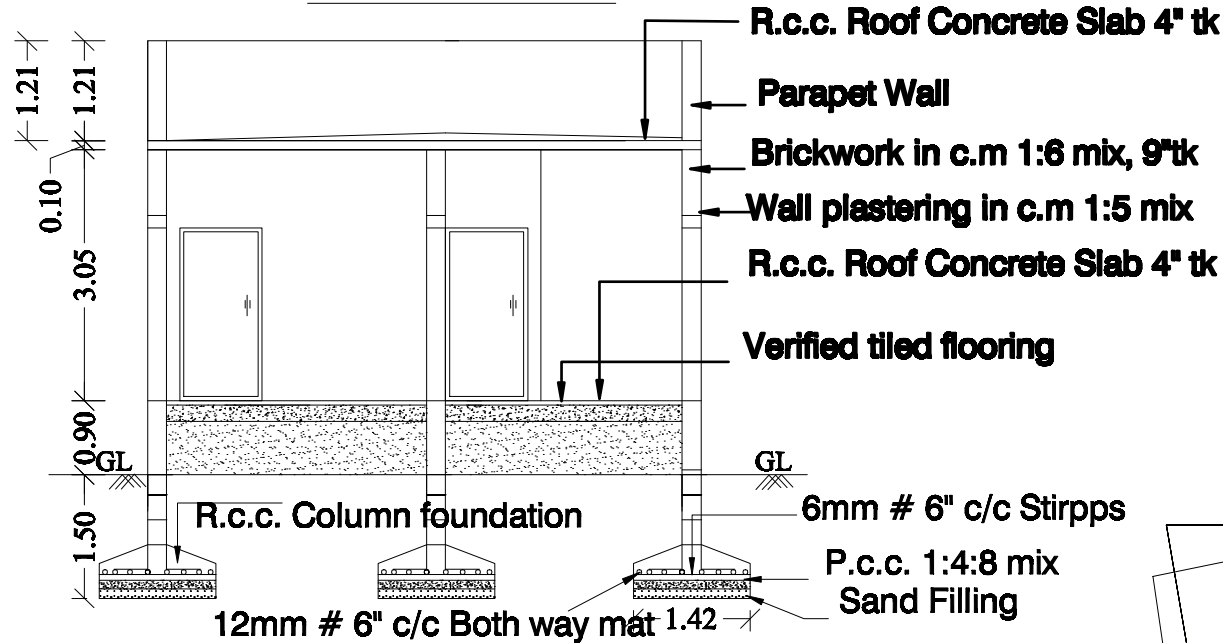
SECTION NN
